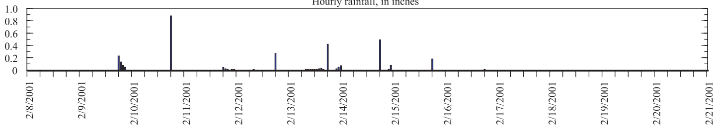
Figure 20. Concentrations of cis-1,2-dichloroethylene and selected continuous monitoring data during a February 2001 storm at Cascade Spring. (Discharge data do not include water captured by Wartrace Water System.)
