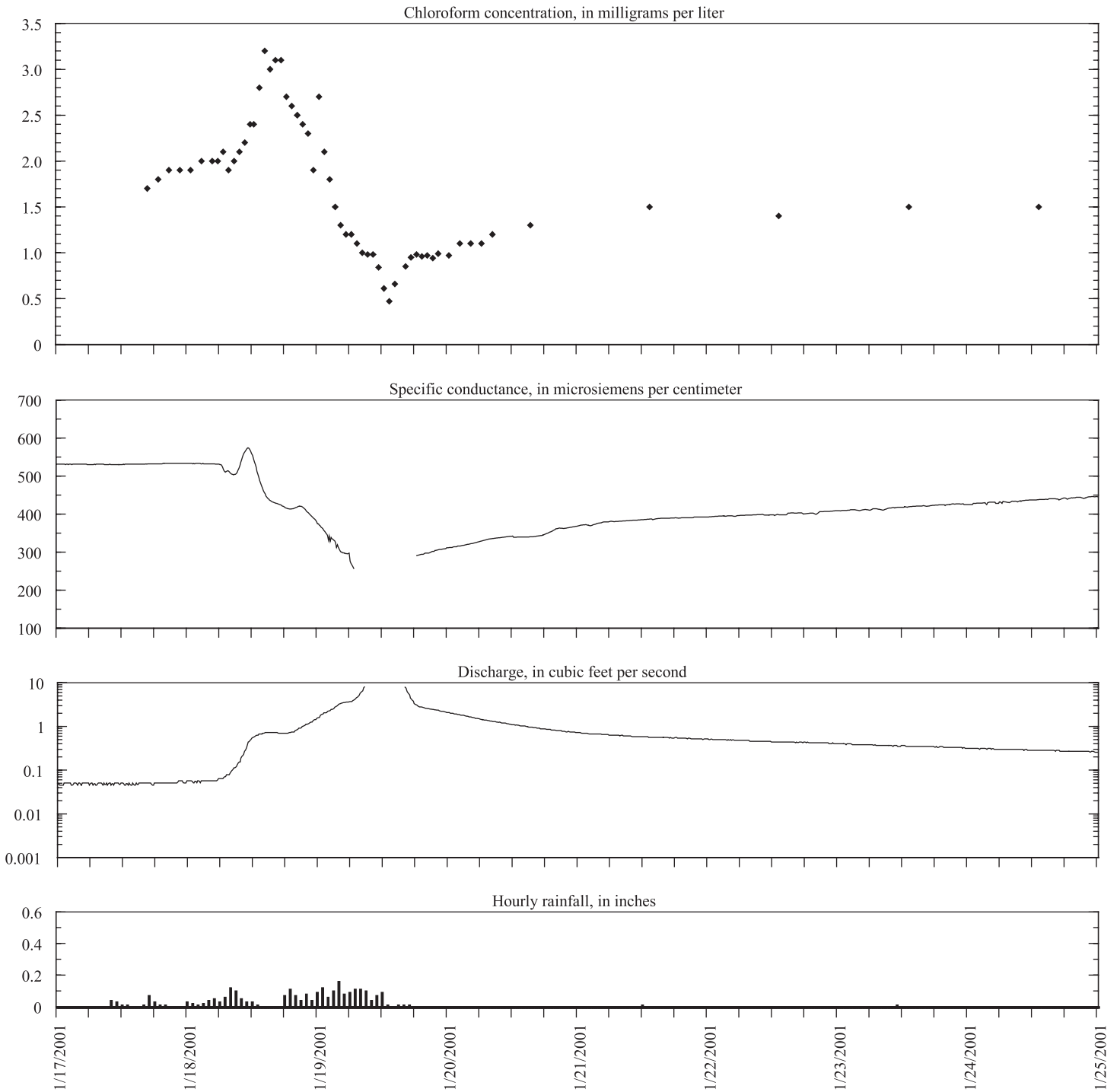
Figure 17. Chloroform concentrations and selected continuous monitoring data during a January 2001 storm at Wilson Spring. (Line gaps indicate missing data.)
